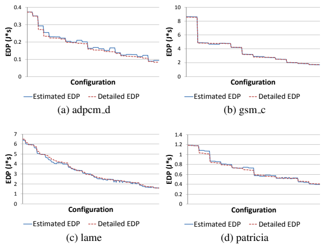
Figure 9: Design space exploration of four benchmarks. Configurations are ordered from high to low EDP values.
