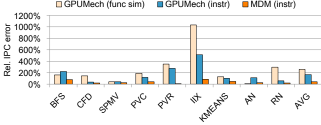
Fig. 10: Hardware validation: relative IPC prediction error for GPU Mech and MDM compared to real hardware. MDM achieves high prediction accuracy compared to real hardware with an average prediction error of 40% compared to 164% for GPU Mech (using binary instrumentation).
