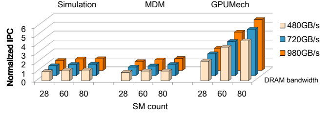
Fig. 12: Normalized performance for CFD as a function of SM count and DRAM bandwidth. All results are normalized to the simulation results at 28 SMs and 480 GB/s DRAM bandwidth. GPU Mech not only leads to high prediction errors, it also over-predicts the performance speedup with more SMs and memory bandwidth, in contrast to MDM.
