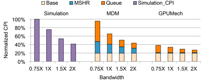
Fig. 14: Normalized CPI as a function of NoC/DRAM bandwidth for the memory-divergent BFS benchmark. MDM accurately captures MSHR batching and NoC/DRAM queueing delays, in contrast to GPUMech.
