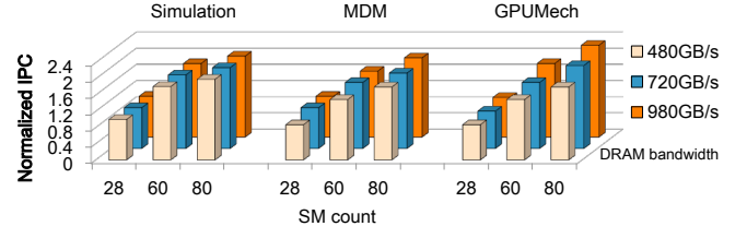
Fig. 11: Normalized performance for BT as a function of SM count and DRAM bandwidth. We normalize to the simulation results at 28 SMs and 480 GB/s DRAM bandwidth. Both GPU Mech and MDM capture the performance trend.
