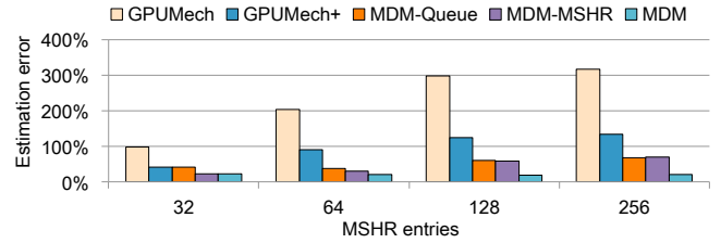
Fig. 8: Prediction error as a function of the number of MSHR entries for the MD-applications.
